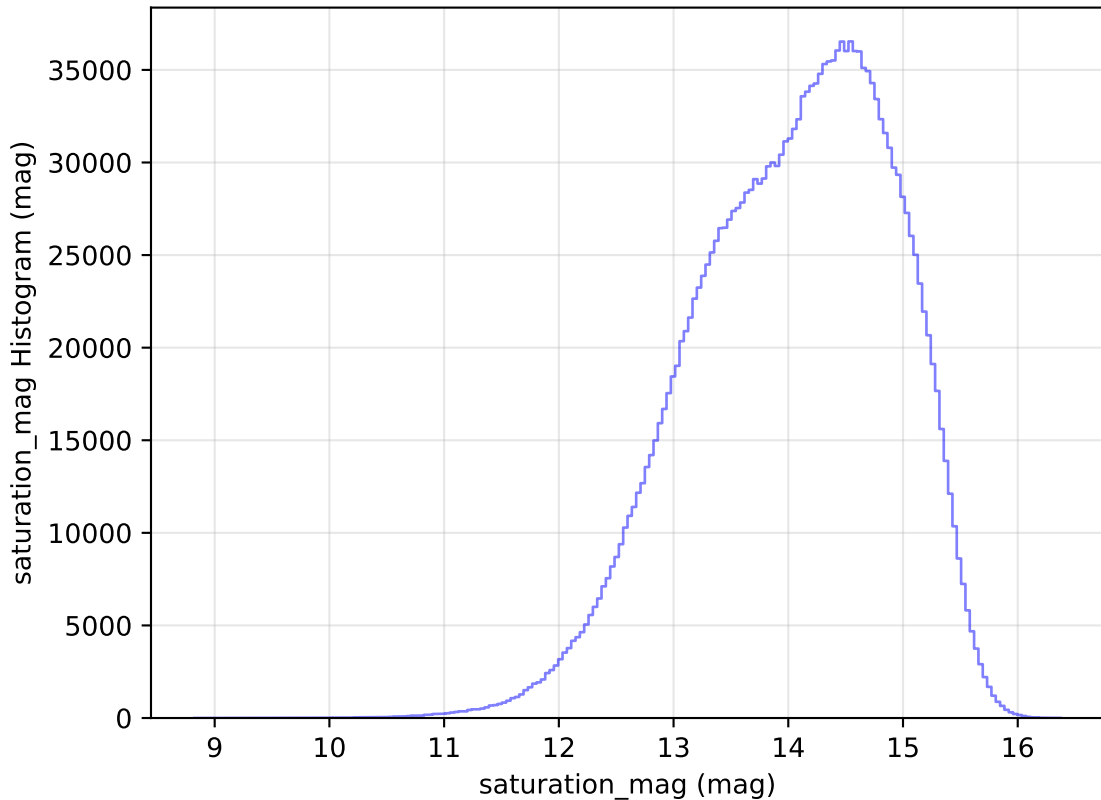
extra_ss_neo3_v3.4_10yrs All sky all bands: saturation_mag Histogram
