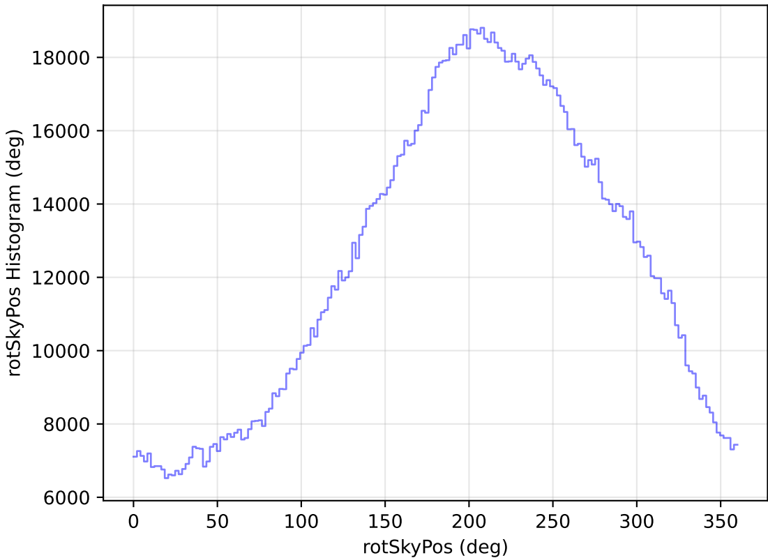
extra_ss_neo3_v3.4_10yrs WFD all bands: rotSkyPos Histogram
