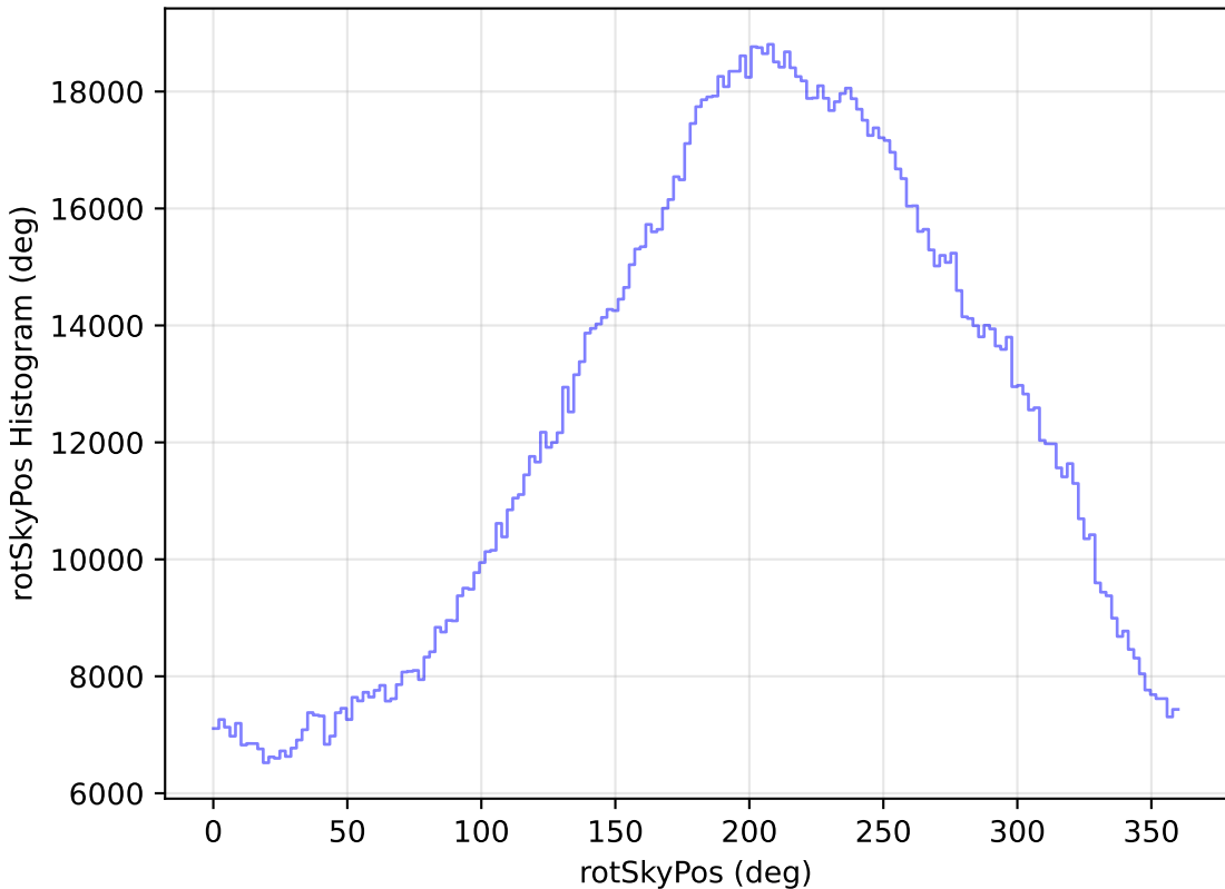
extra_ss_neo3_v3.4_10yrs All sky all bands: rotSkyPos Histogram
