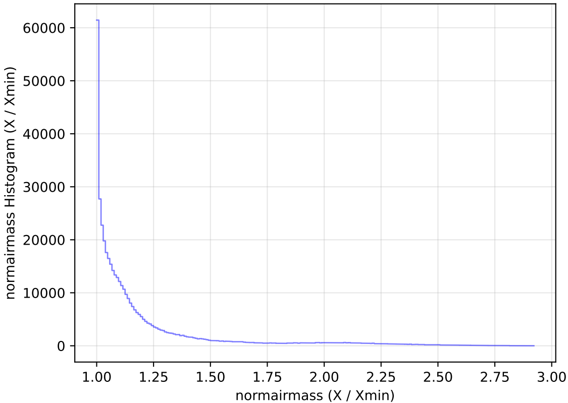
extra_ss_neo3_v3.4_10yrs WFD z band: normairmass Histogram
