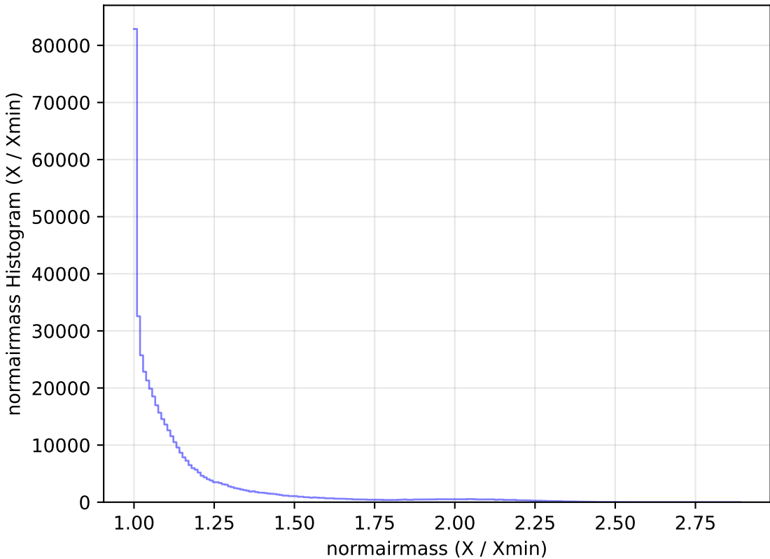
extra_ss_neo3_v3.4_10yrs WFD r band: normairmass Histogram
