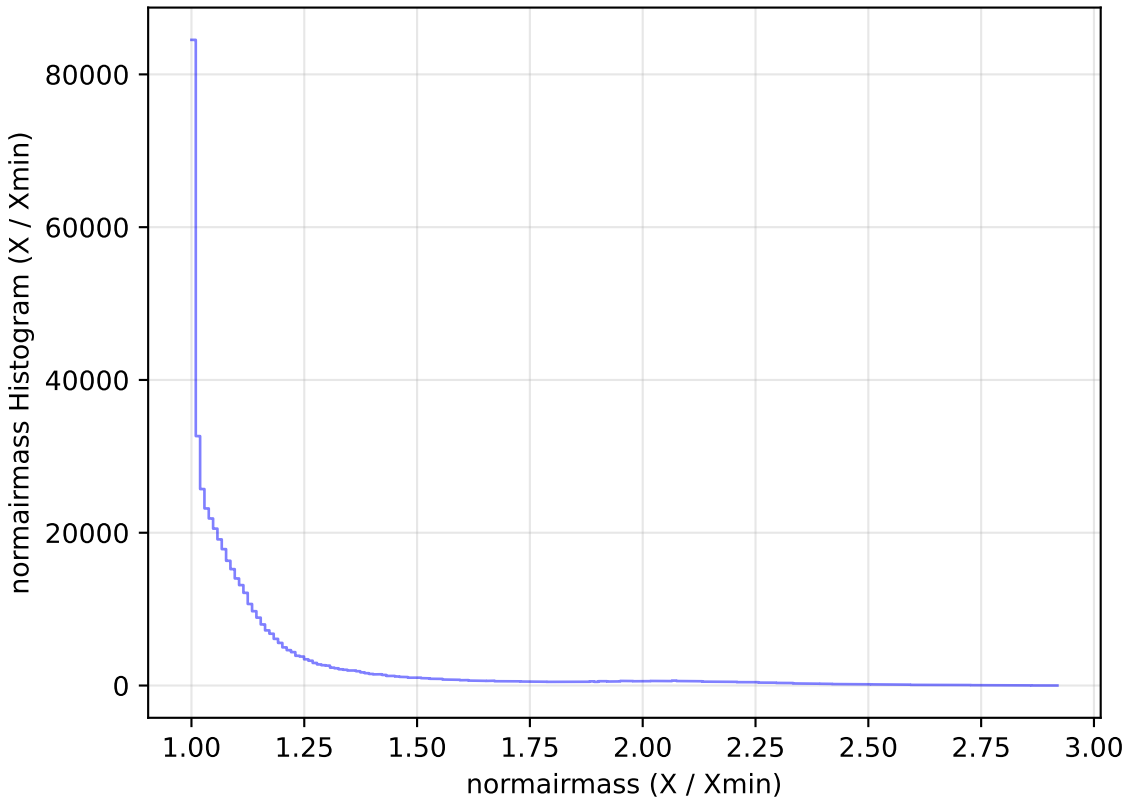
extra_ss_neo3_v3.4_10yrs WFD i band: normairmass Histogram
