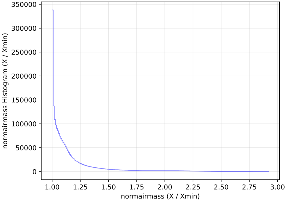
extra_ss_neo3_v3.4_10yrs WFD all bands: normairmass Histogram
