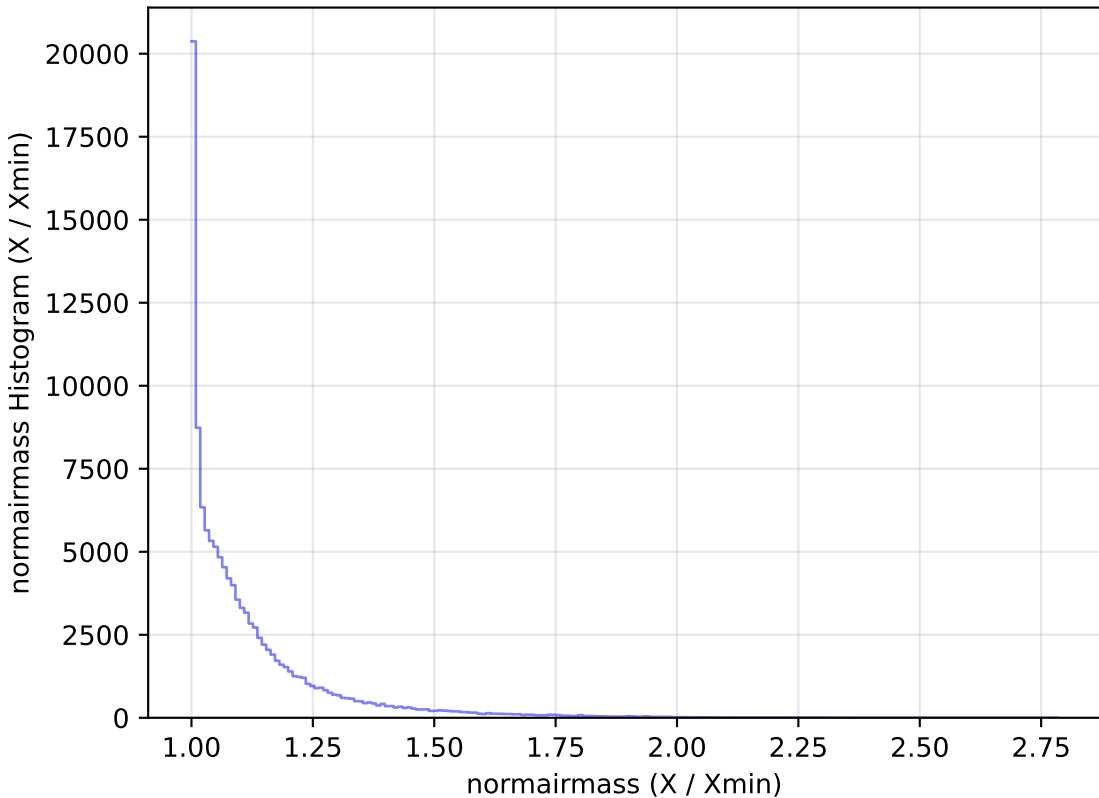
extra_ss_neo3_v3.4_10yrs All sky u band: normairmass Histogram
