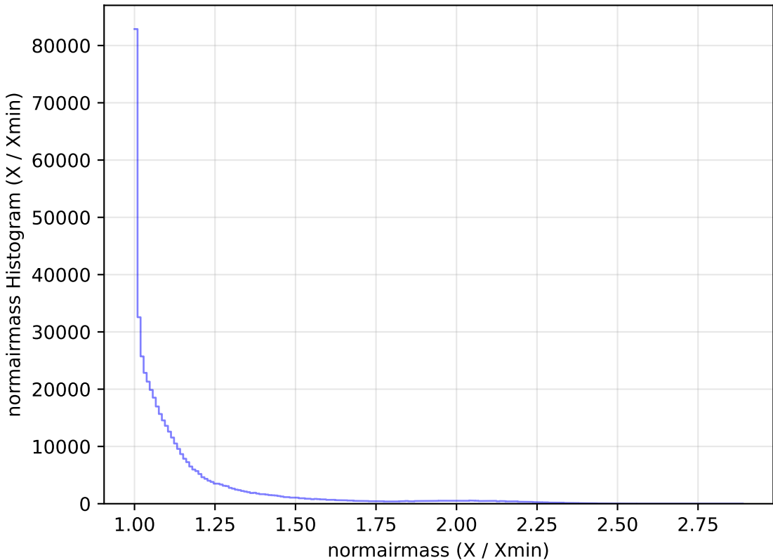
extra_ss_neo3_v3.4_10yrs All sky r band: normairmass Histogram
