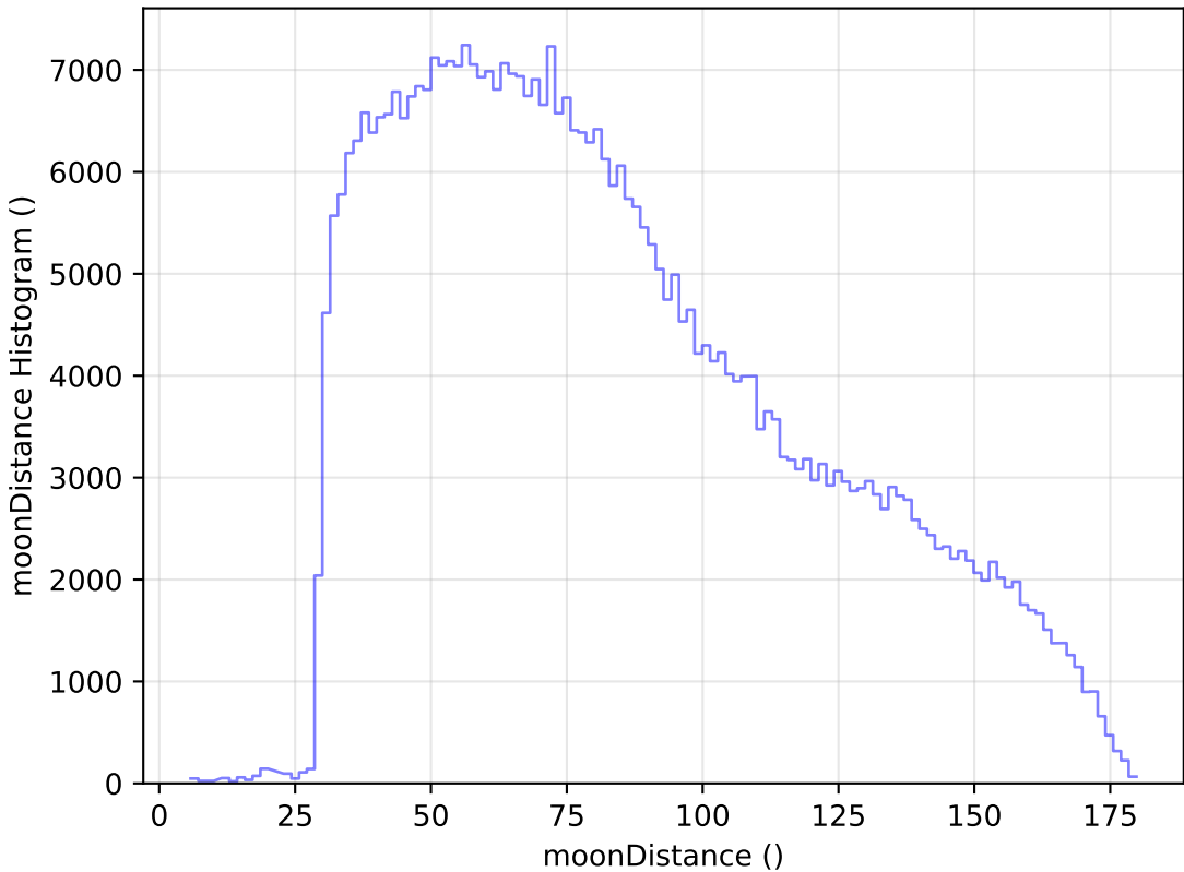
extra_ss_neo3_v3.4_10yrs WFD z band: moonDistance Histogram
