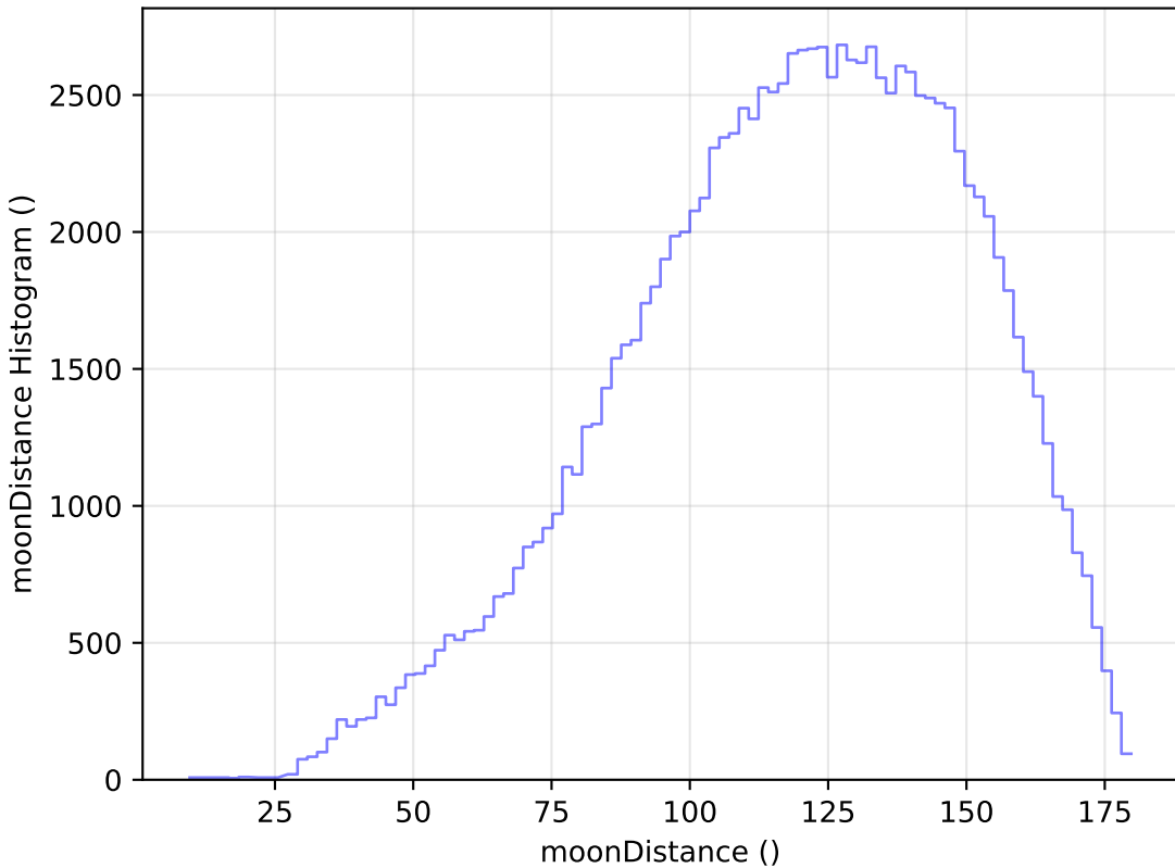
extra_ss_neo3_v3.4_10yrs WFD u band: moonDistance Histogram
