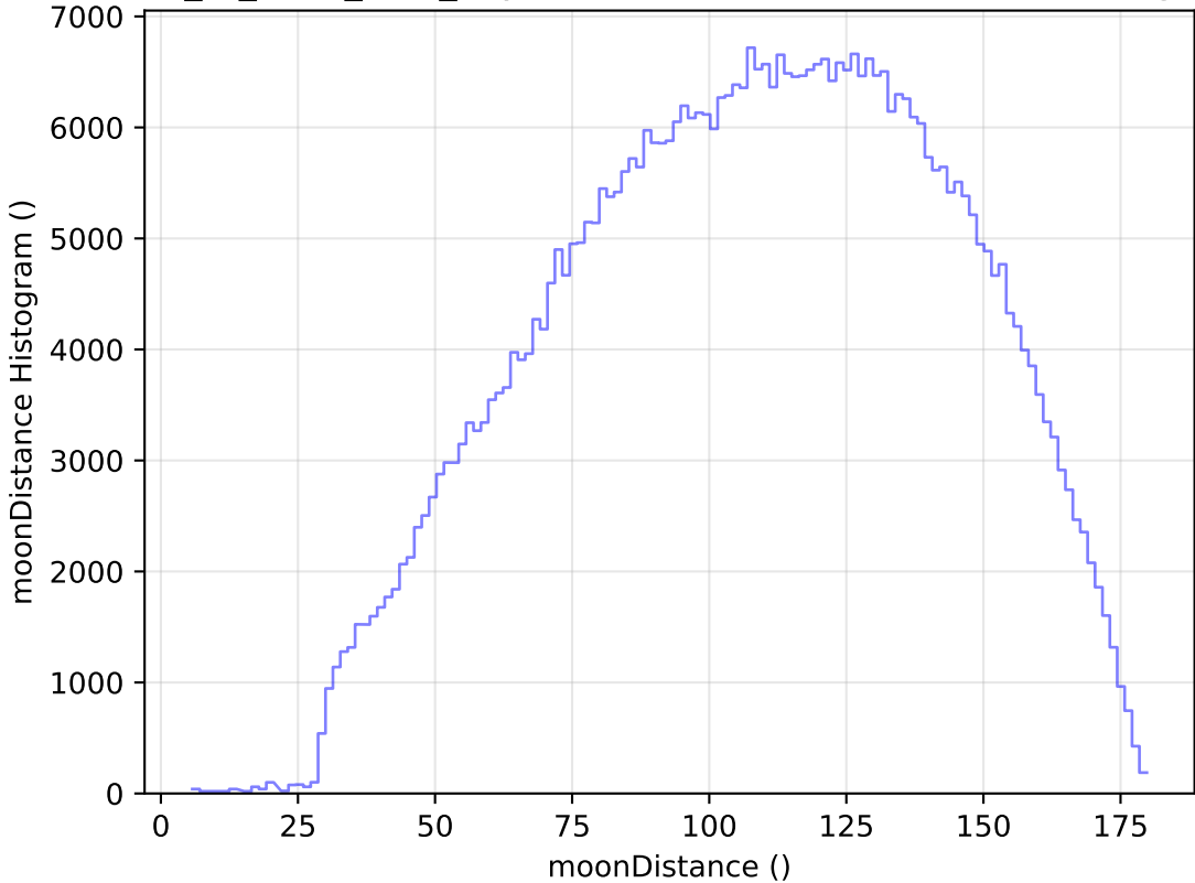
extra_ss_neo3_v3.4_10yrs WFD r band: moonDistance Histogram
