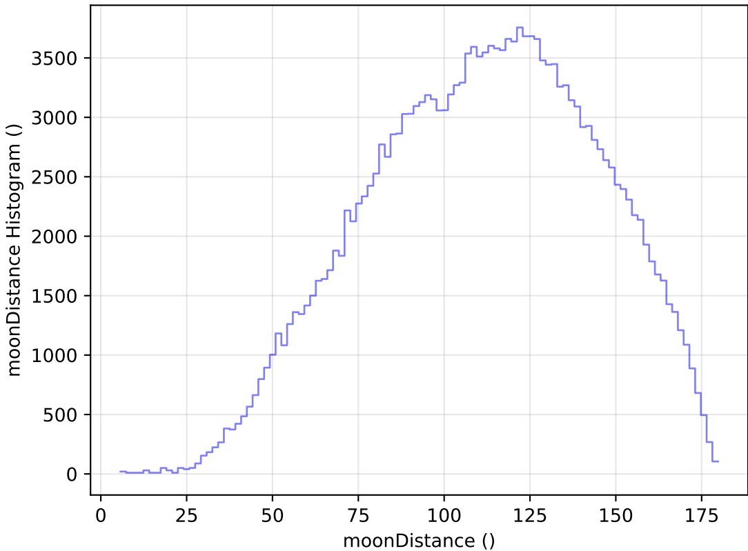
extra_ss_neo3_v3.4_10yrs WFD g band: moonDistance Histogram
