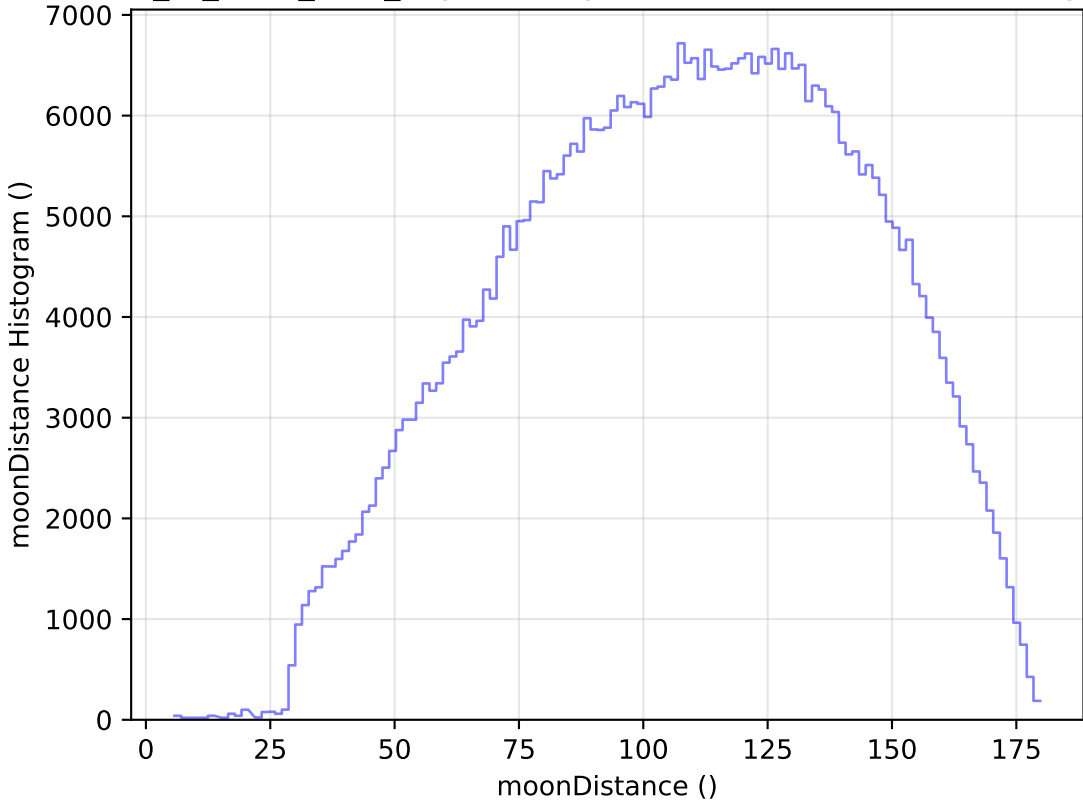
extra_ss_neo3_v3.4_10yrs All sky r band: moonDistance Histogram
