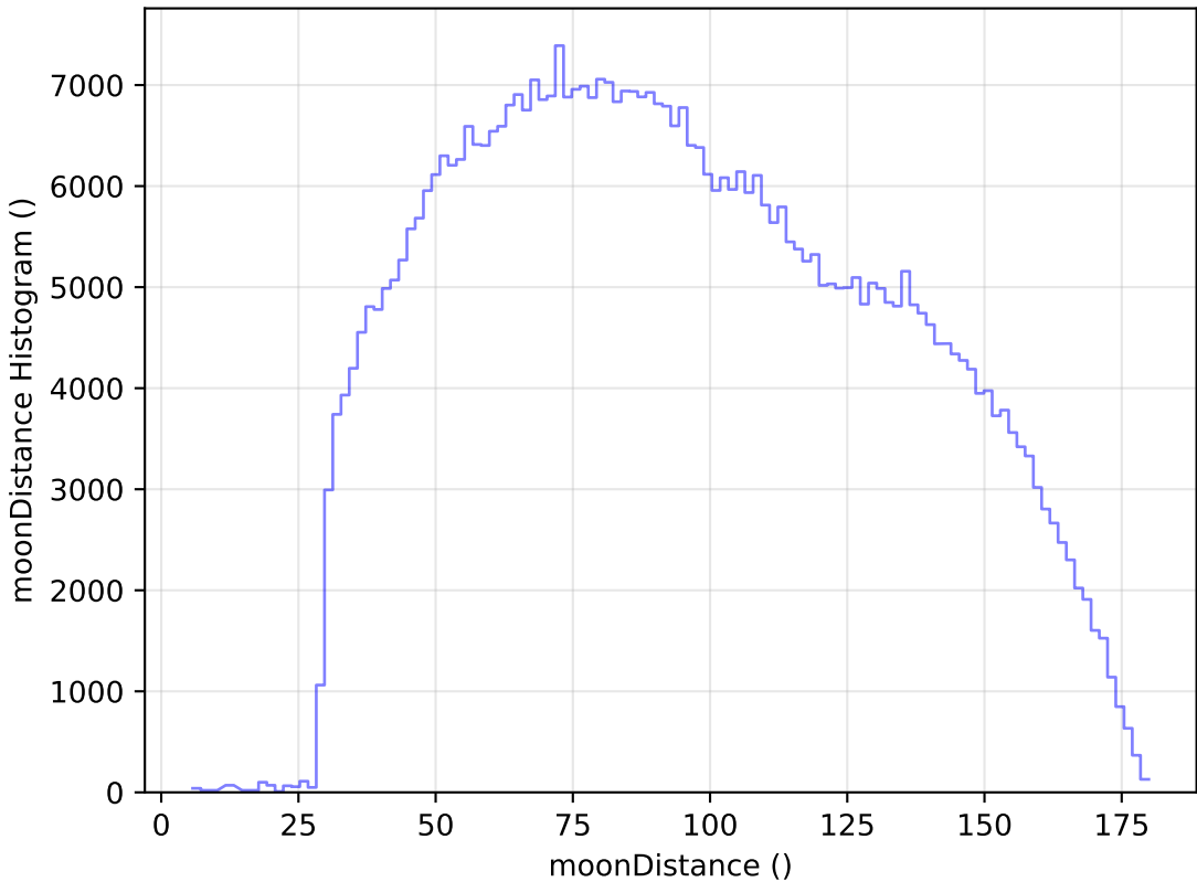
extra_ss_neo3_v3.4_10yrs All sky i band: moonDistance Histogram
