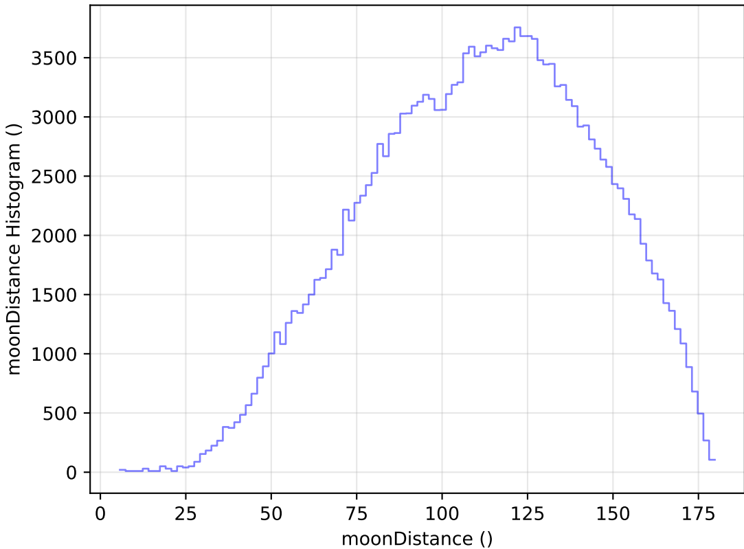
extra_ss_neo3_v3.4_10yrs All sky g band: moonDistance Histogram
