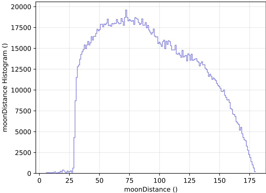
extra_ss_neo3_v3.4_10yrs All sky all bands: moonDistance Histogram
