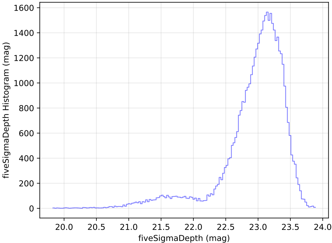
extra_ss_neo3_v3.4_10yrs Yr 1 z band: fiveSigmaDepth Histogram
