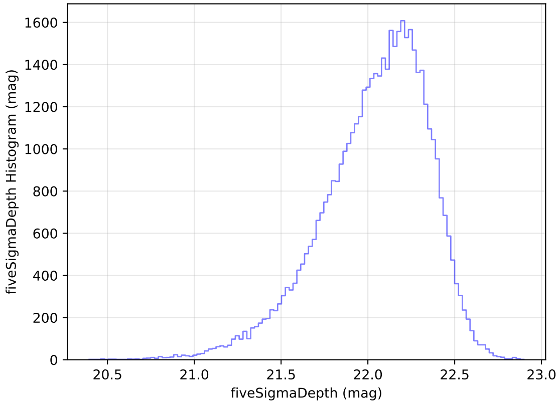
extra_ss_neo3_v3.4_10yrs Yr 1 y band: fiveSigmaDepth Histogram
