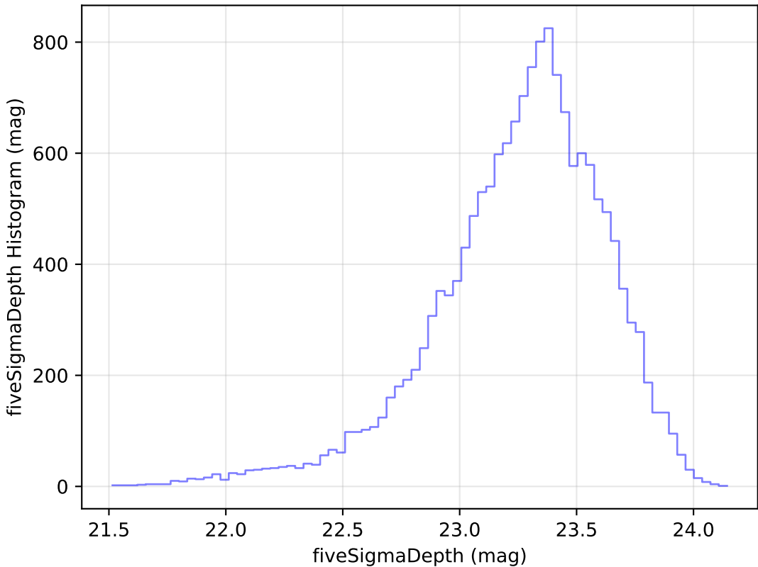
extra_ss_neo3_v3.4_10yrs Yr 1 u band: fiveSigmaDepth Histogram
