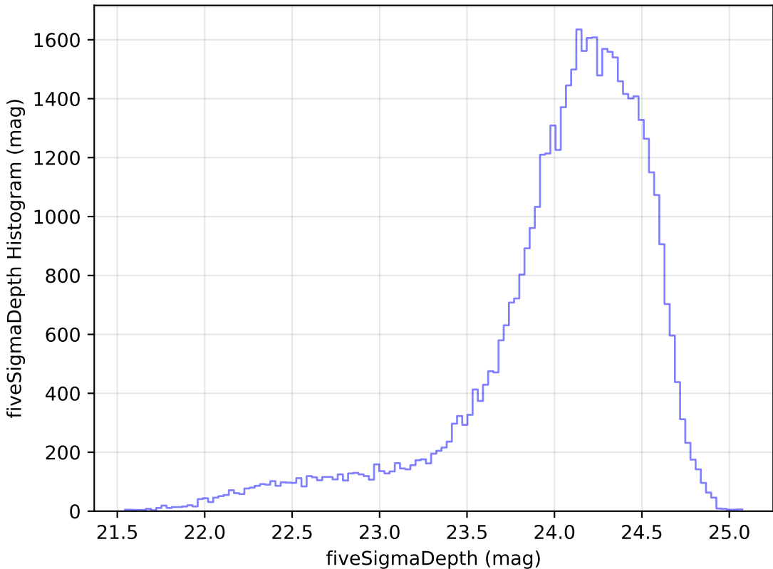
extra_ss_neo3_v3.4_10yrs Yr 1 r band: fiveSigmaDepth Histogram
