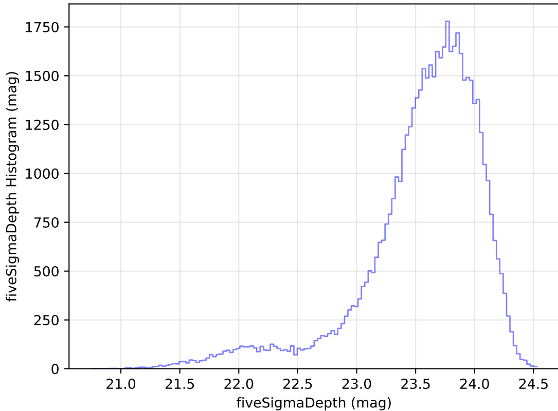
extra_ss_neo3_v3.4_10yrs Yr 1 i band: fiveSigmaDepth Histogram
