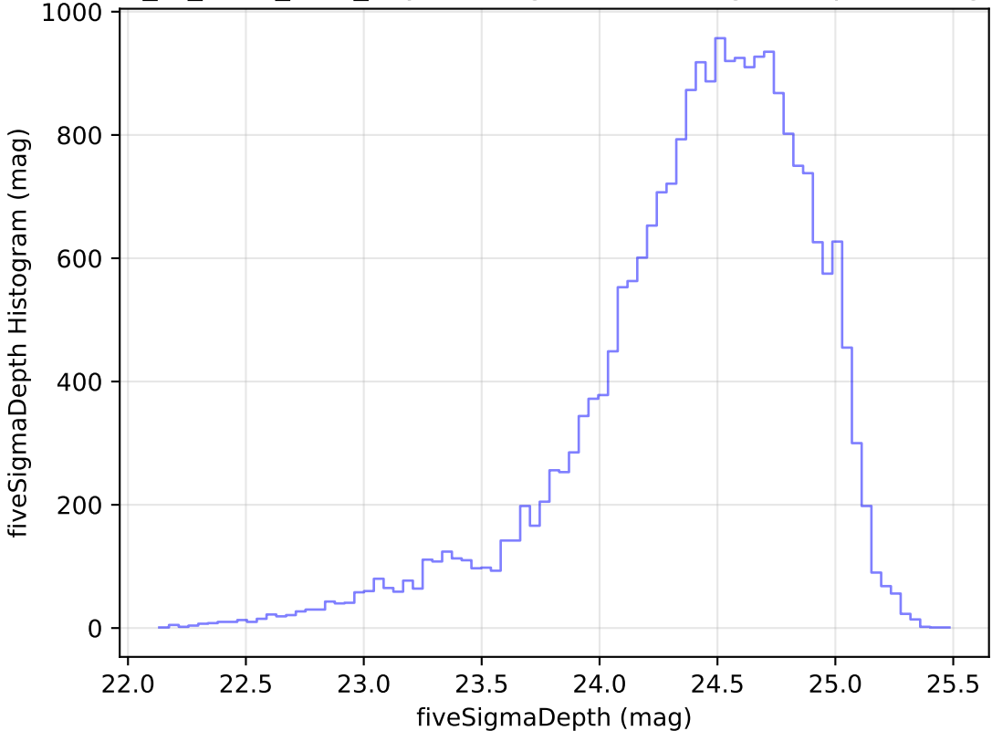
extra_ss_neo3_v3.4_10yrs Yr 1 g band: fiveSigmaDepth Histogram
