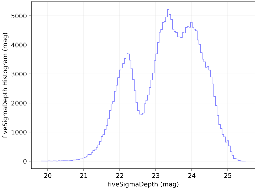
extra_ss_neo3_v3.4_10yrs Yr 1 all bands: fiveSigmaDepth Histogram
