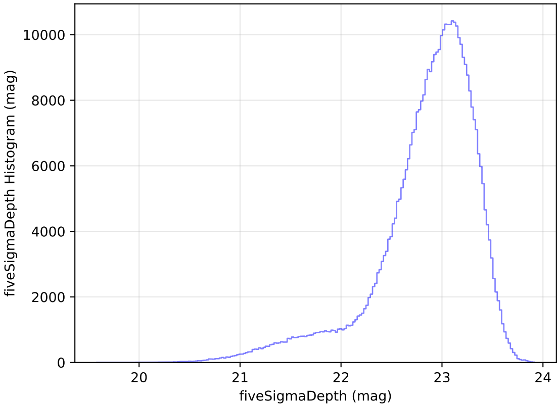
extra_ss_neo3_v3.4_10yrs WFD z band: fiveSigmaDepth Histogram
