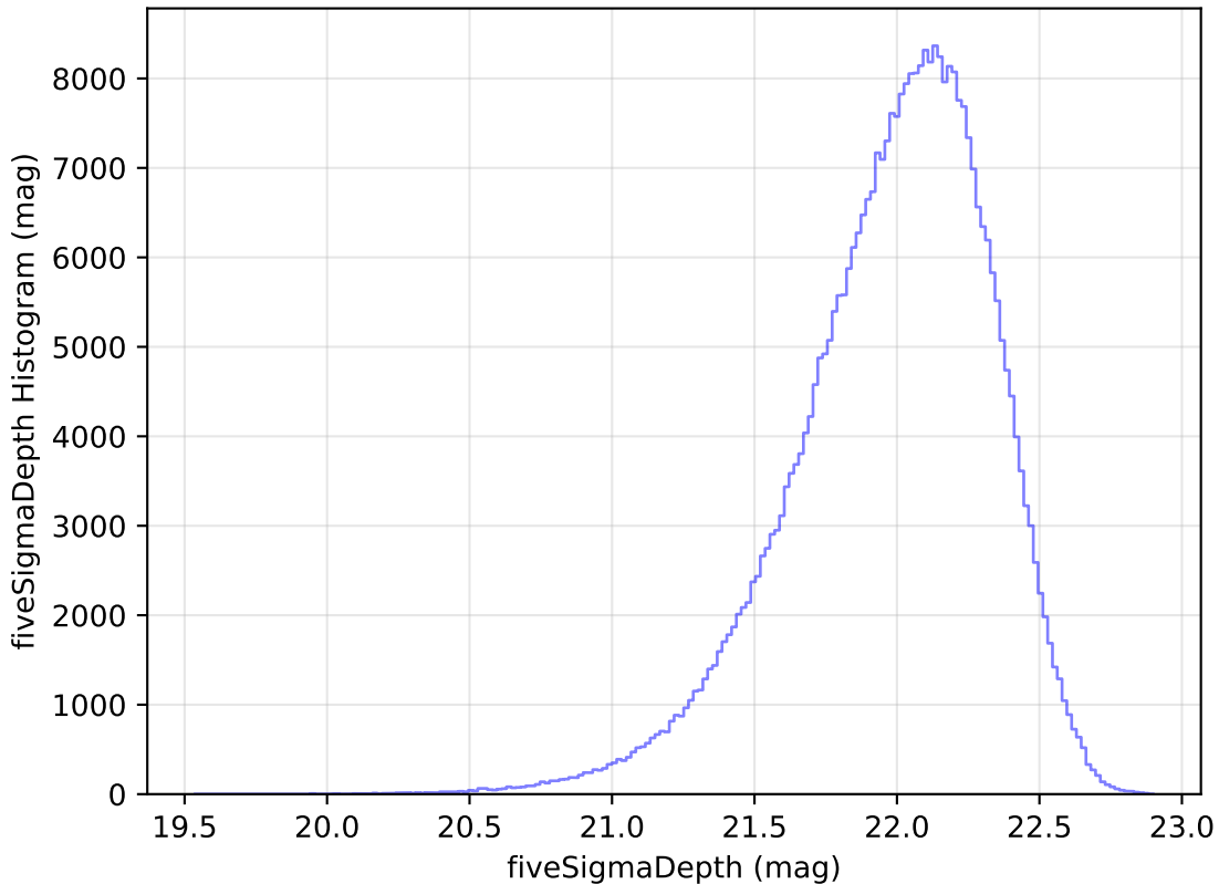
extra_ss_neo3_v3.4_10yrs WFD y band: fiveSigmaDepth Histogram
