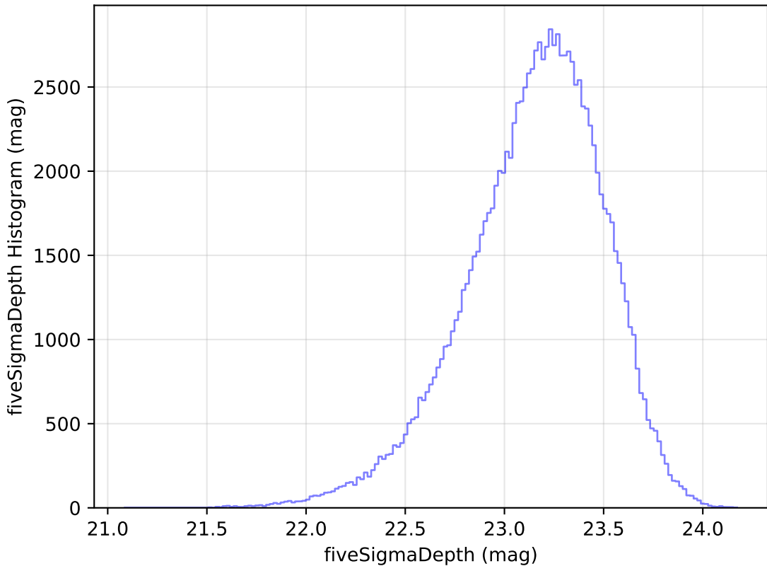
extra_ss_neo3_v3.4_10yrs WFD u band: fiveSigmaDepth Histogram
