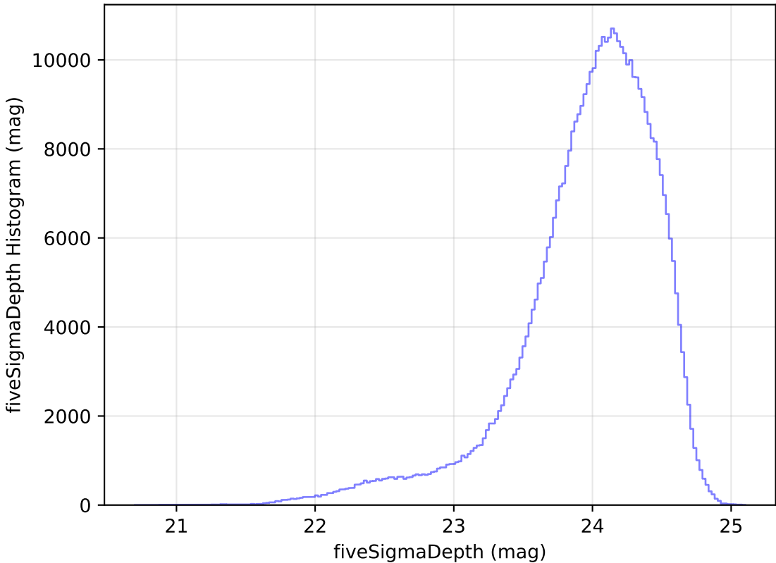
extra_ss_neo3_v3.4_10yrs WFD r band: fiveSigmaDepth Histogram
