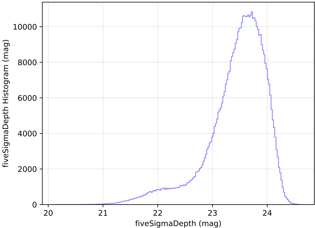
extra_ss_neo3_v3.4_10yrs WFD i band: fiveSigmaDepth Histogram
