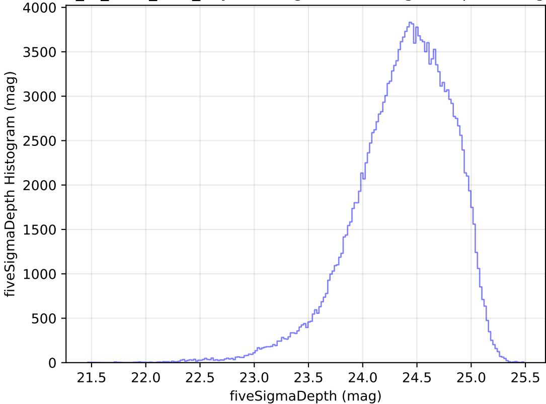
extra_ss_neo3_v3.4_10yrs WFD g band: fiveSigmaDepth Histogram
