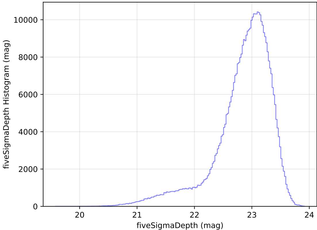
extra_ss_neo3_v3.4_10yrs All sky z band: fiveSigmaDepth Histogram
