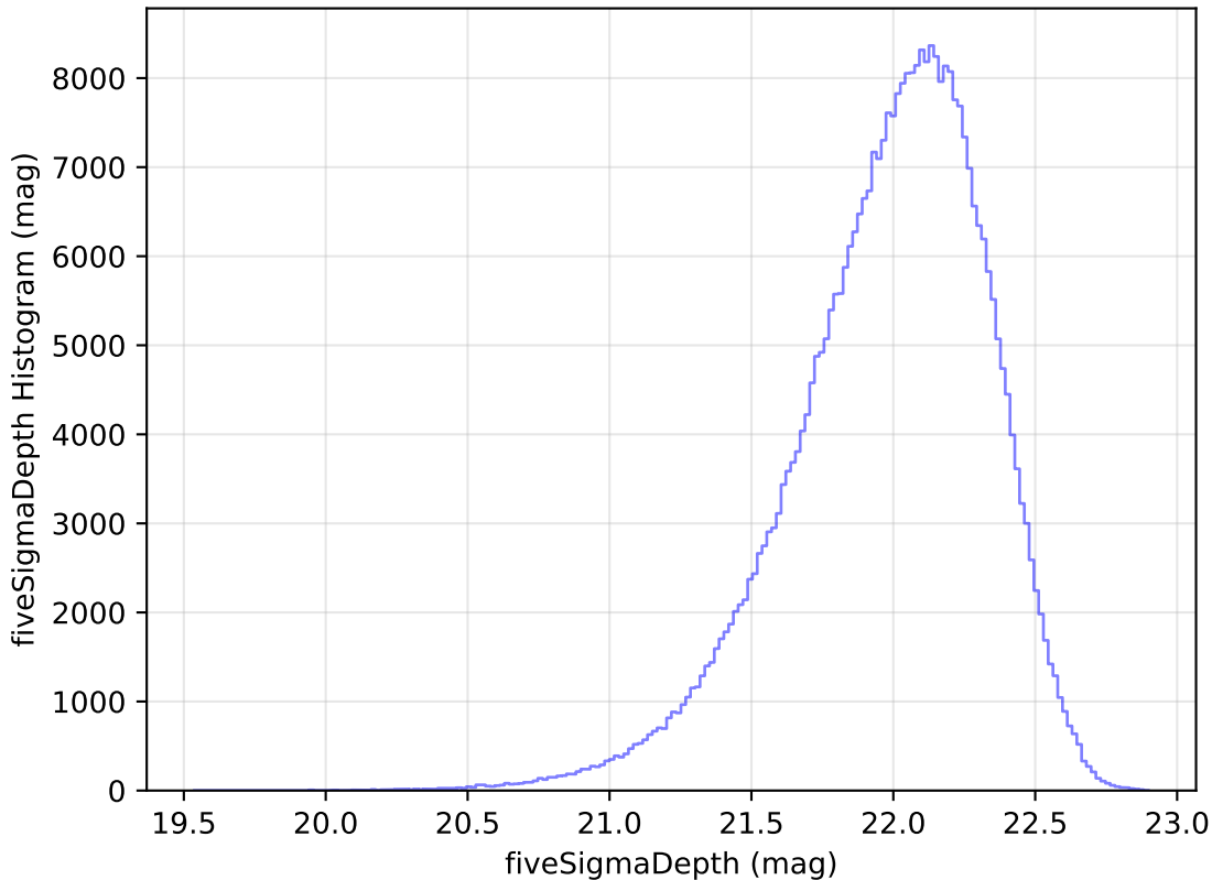
extra_ss_neo3_v3.4_10yrs All sky y band: fiveSigmaDepth Histogram
