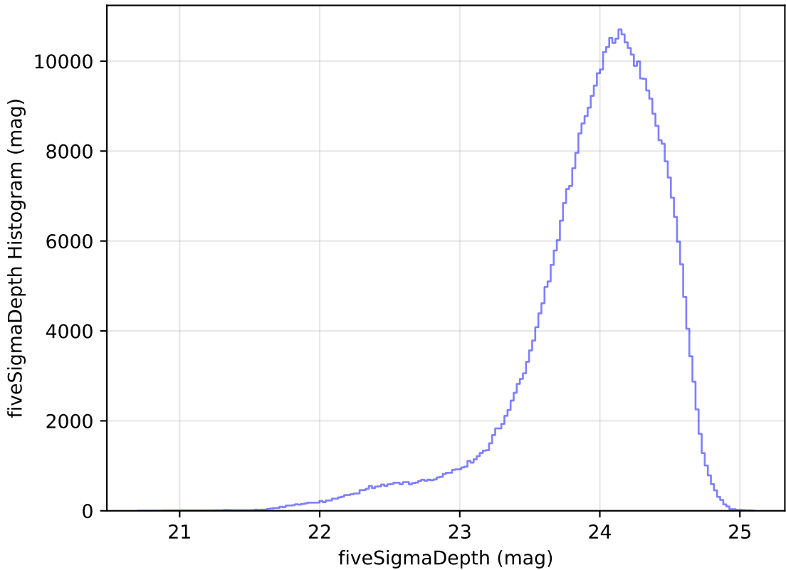
extra_ss_neo3_v3.4_10yrs All sky r band: fiveSigmaDepth Histogram
