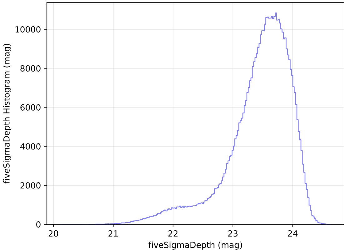
extra_ss_neo3_v3.4_10yrs All sky i band: fiveSigmaDepth Histogram
