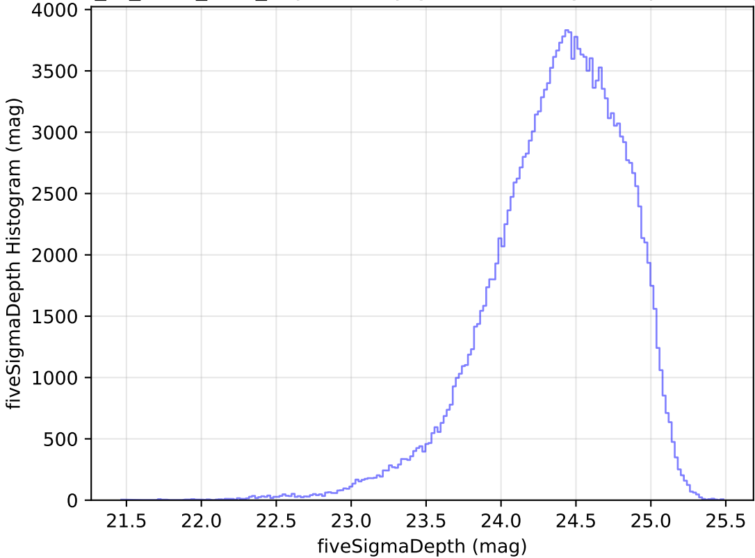
extra_ss_neo3_v3.4_10yrs All sky g band: fiveSigmaDepth Histogram
