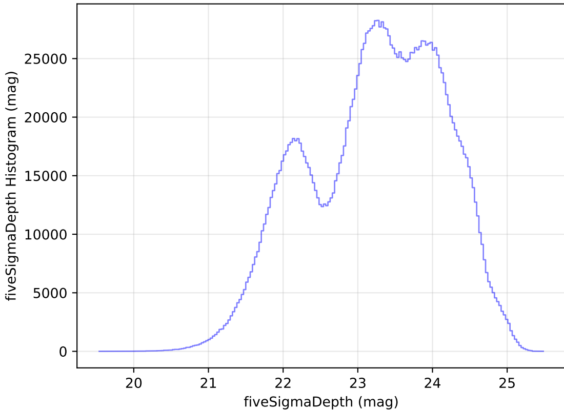
extra_ss_neo3_v3.4_10yrs All sky all bands: fiveSigmaDepth Histogram
