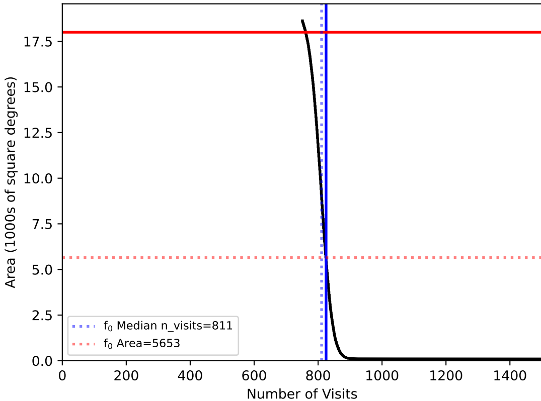
extra_ss_neo3_v3.4_10yrs WFD: fO
