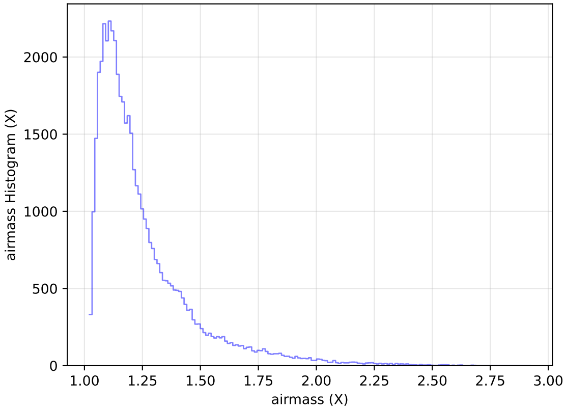
extra_ss_neo3_v3.4_10yrs Yr 1 y band: airmass Histogram
