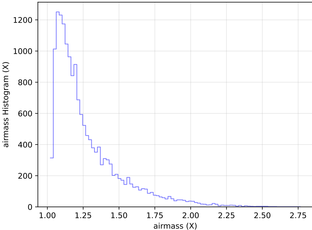
extra_ss_neo3_v3.4_10yrs Yr 1 u band: airmass Histogram
