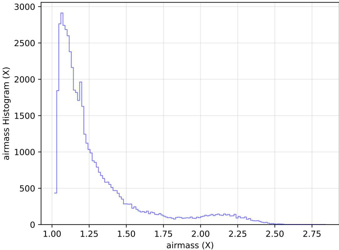
extra_ss_neo3_v3.4_10yrs Yr 1 r band: airmass Histogram
