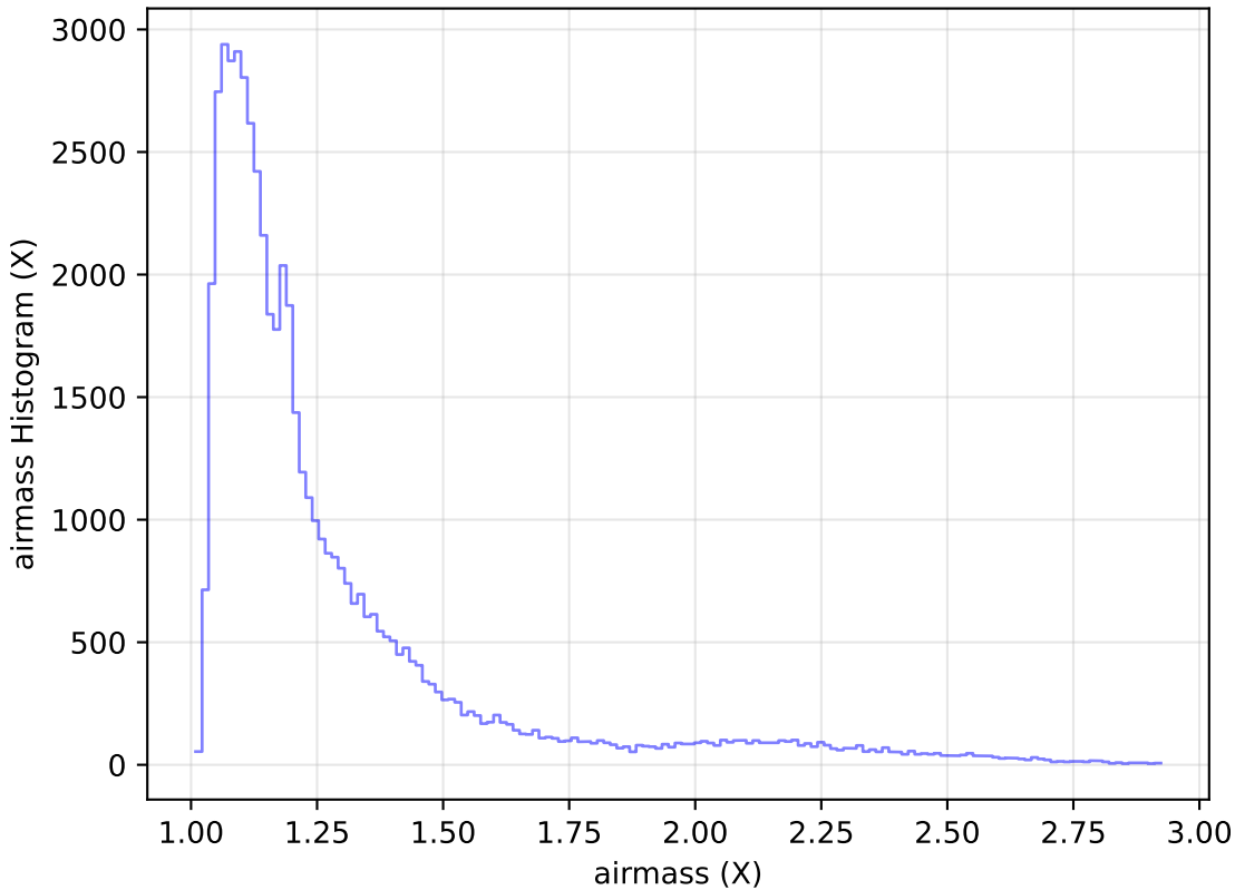
extra_ss_neo3_v3.4_10yrs Yr 1 i band: airmass Histogram
