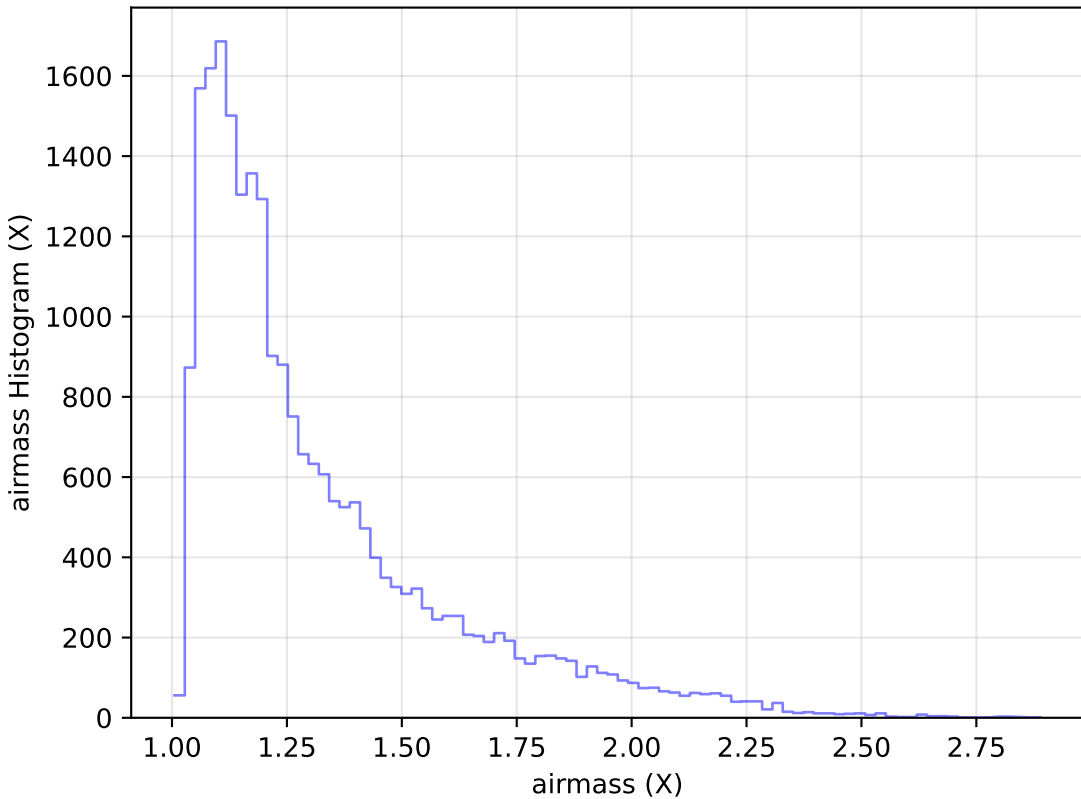
extra_ss_neo3_v3.4_10yrs Yr 1 g band: airmass Histogram
