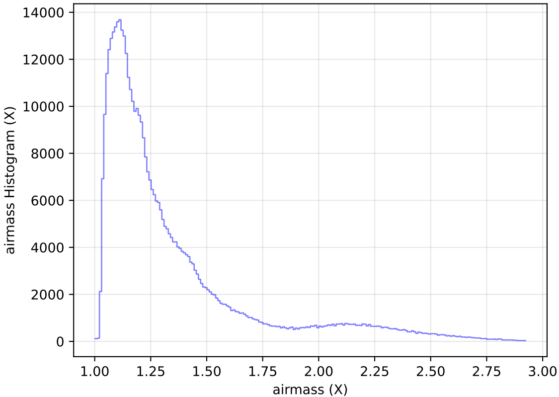
extra_ss_neo3_v3.4_10yrs WFD z band: airmass Histogram
