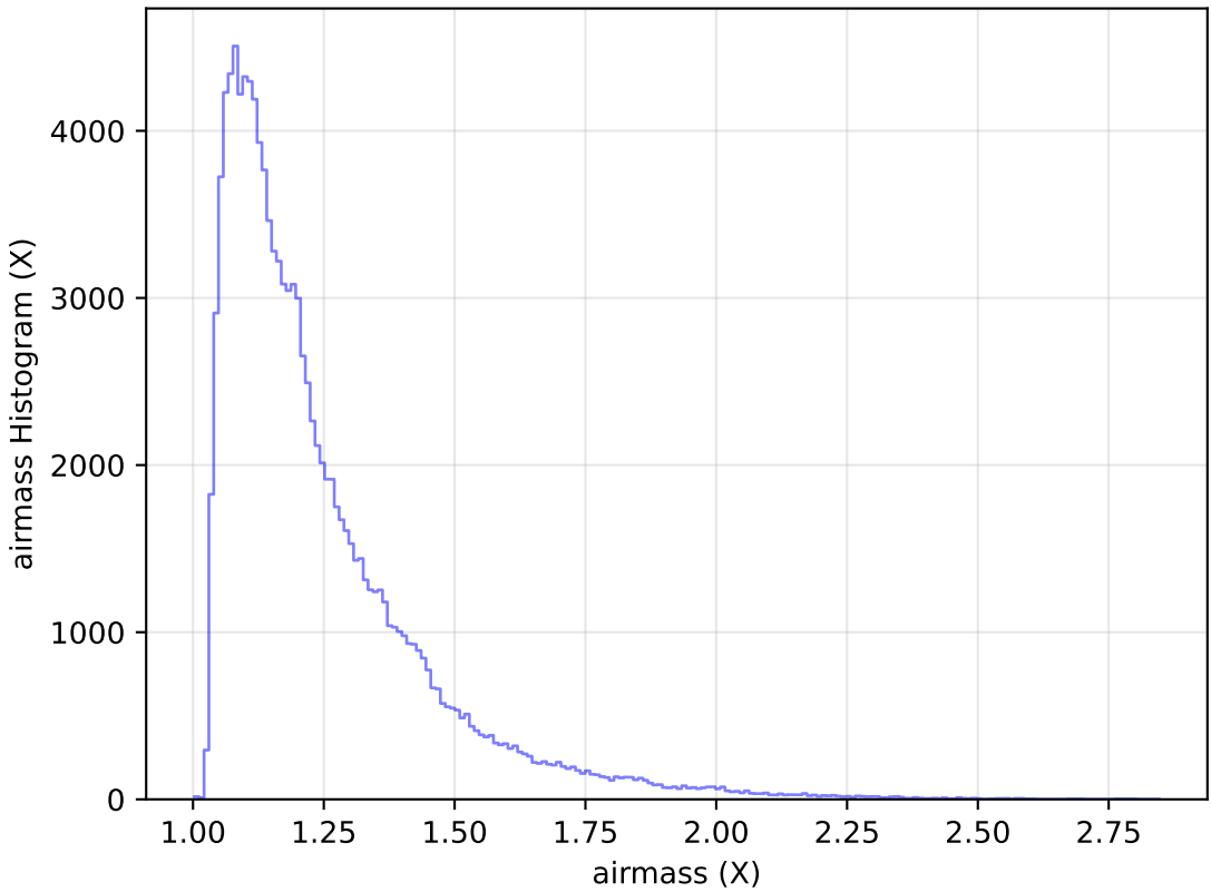
extra_ss_neo3_v3.4_10yrs WFD u band: airmass Histogram
