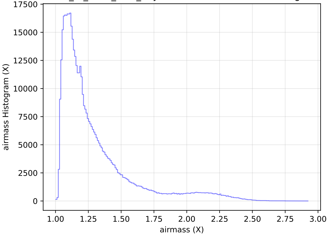
extra_ss_neo3_v3.4_10yrs WFD r band: airmass Histogram
