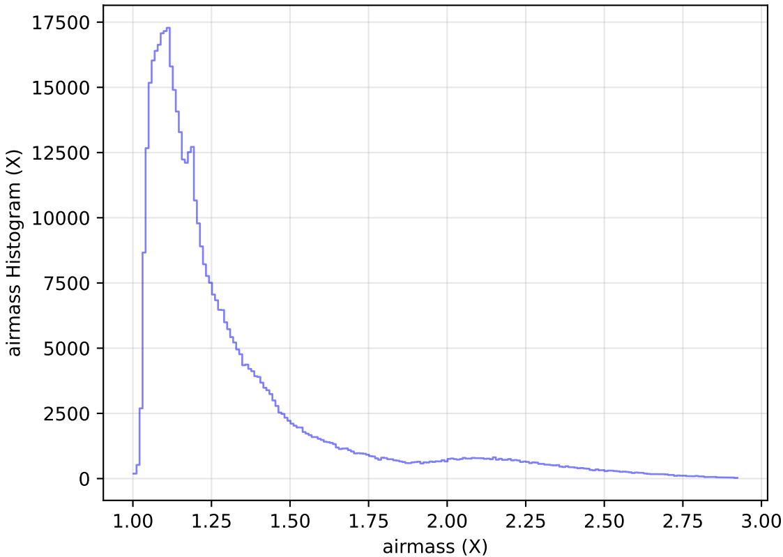
extra_ss_neo3_v3.4_10yrs WFD i band: airmass Histogram
