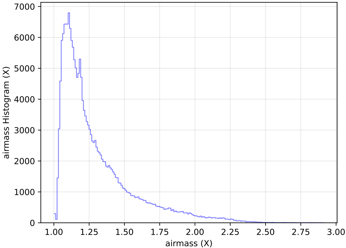
extra_ss_neo3_v3.4_10yrs WFD g band: airmass Histogram
