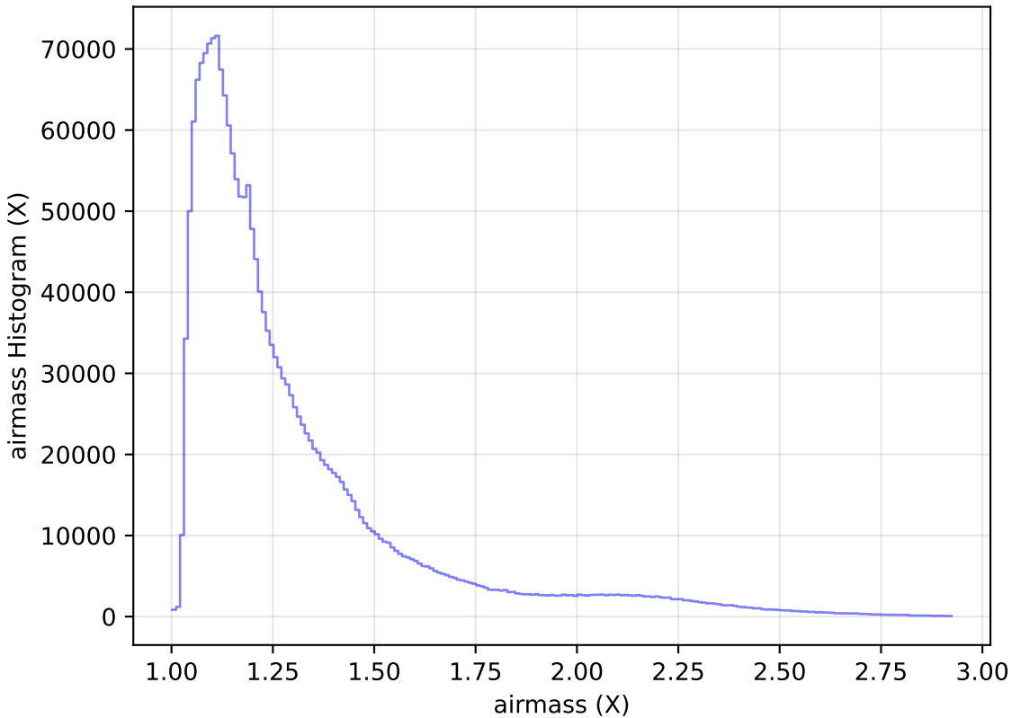
extra_ss_neo3_v3.4_10yrs WFD all bands: airmass Histogram
