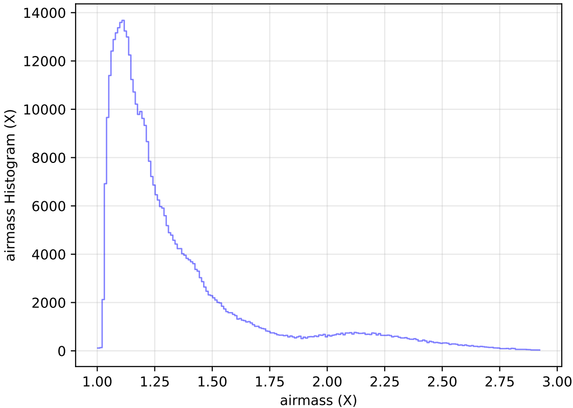
extra_ss_neo3_v3.4_10yrs All sky z band: airmass Histogram
