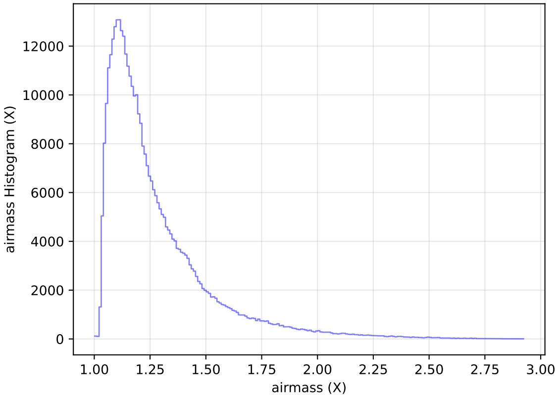
extra_ss_neo3_v3.4_10yrs All sky y band: airmass Histogram
